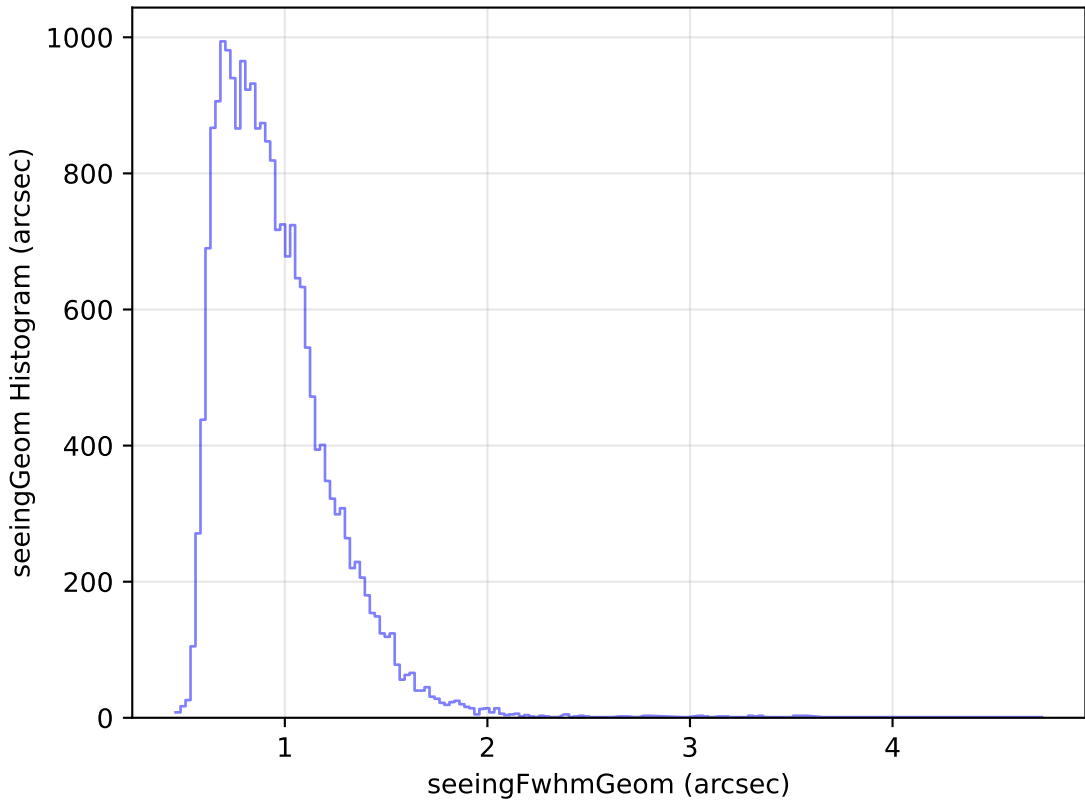
ddf_loaded_half_fl2_v3.4_10yrs Yr 1 g band: seeingGeom Histogram
