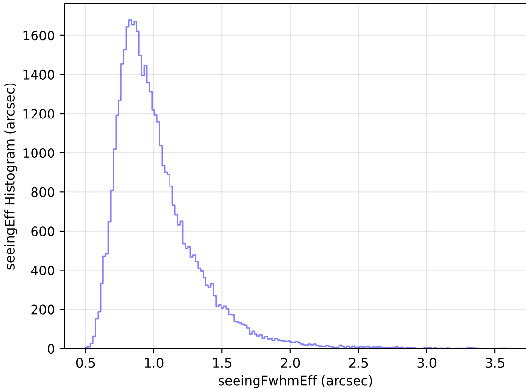
ddf_loaded_half_fl2_v3.4_10yrs Yr 1 z band: seeingEff Histogram
