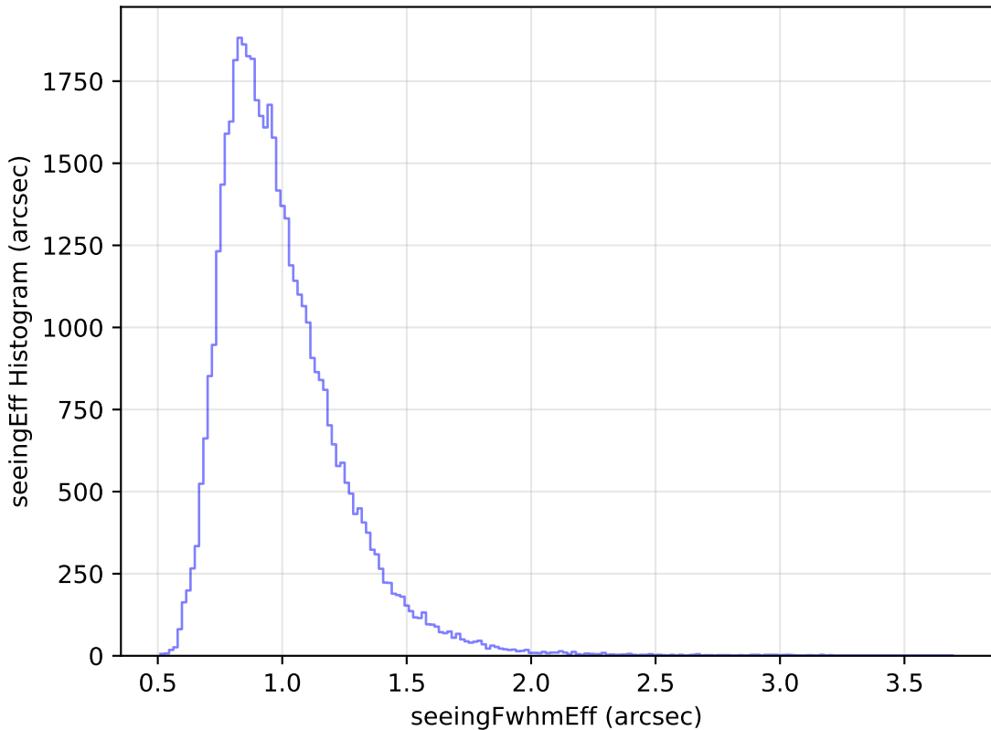
ddf_loaded_half_fl2_v3.4_10yrs Yr 1 y band: seeingEff Histogram
