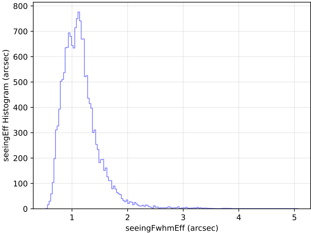
ddf_loaded_half_fl2_v3.4_10yrs Yr 1 u band: seeingEff Histogram
