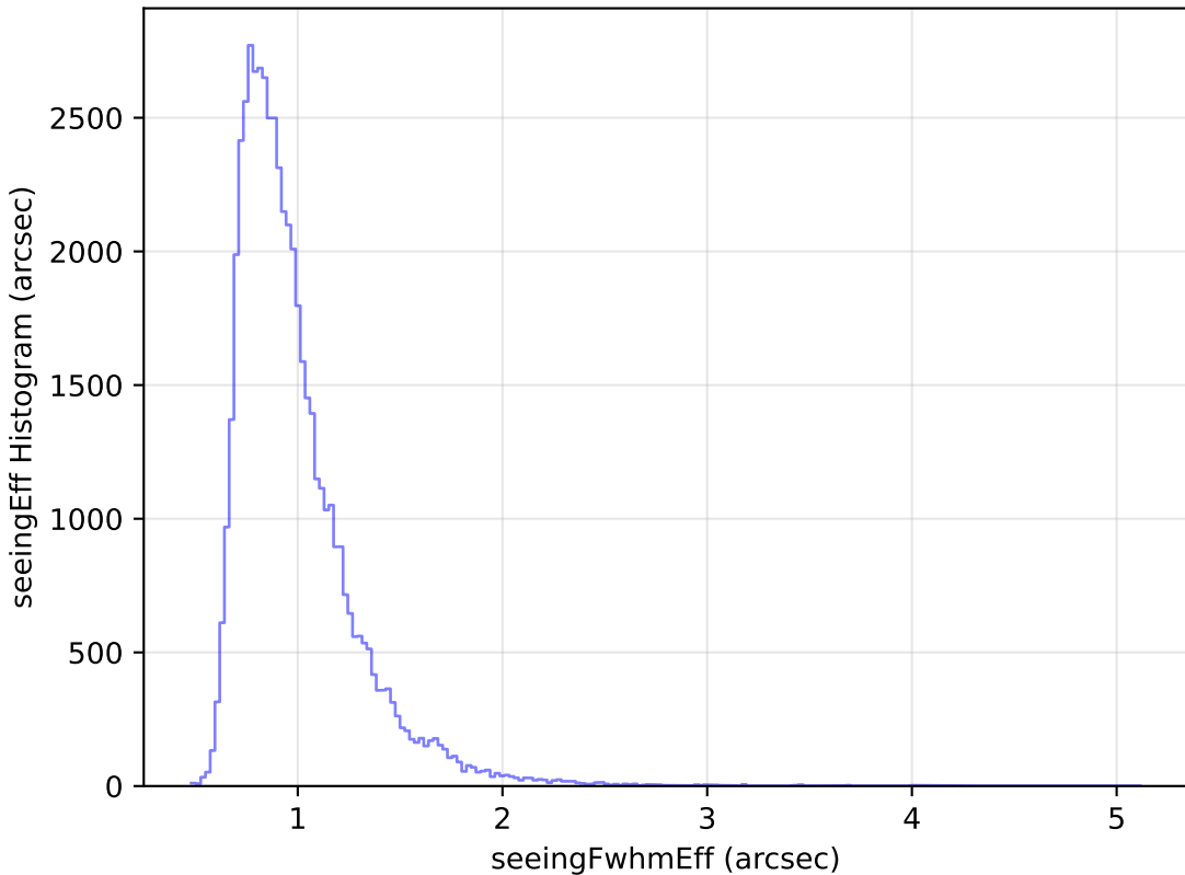
ddf_loaded_half_fl2_v3.4_10yrs Yr 1 i band: seeingEff Histogram
