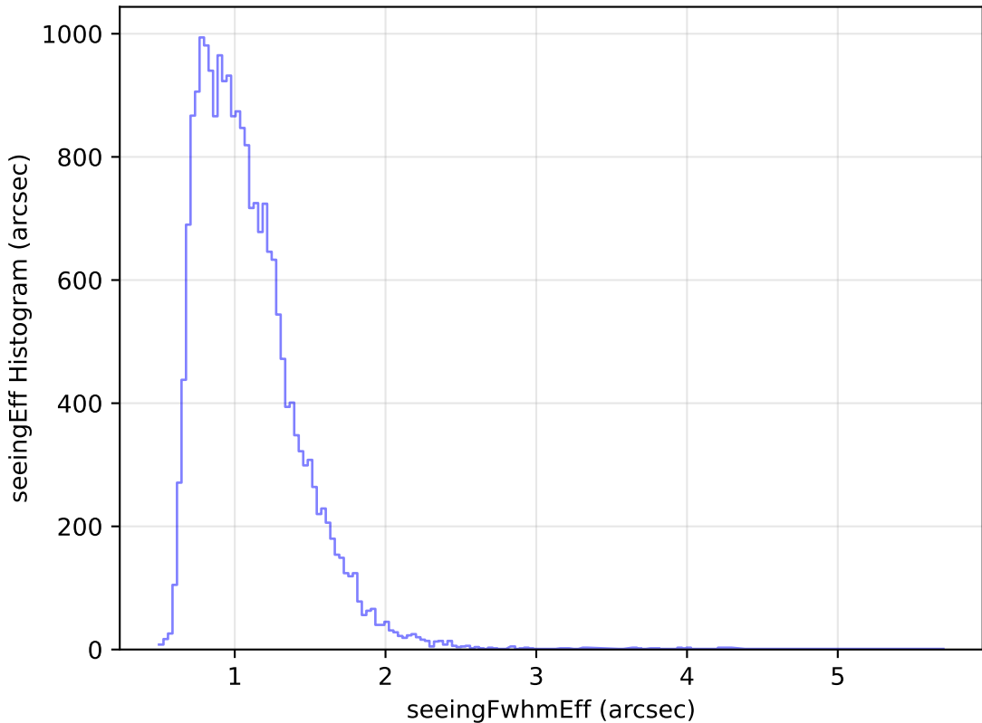
ddf_loaded_half_fl2_v3.4_10yrs Yr 1 g band: seeingEff Histogram
