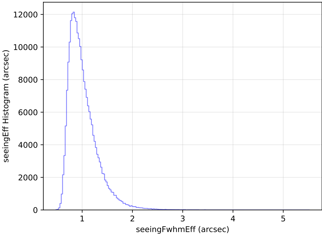
ddf_loaded_half_fl2_v3.4_10yrs Yr 1 all bands: seeingEff Histogram
