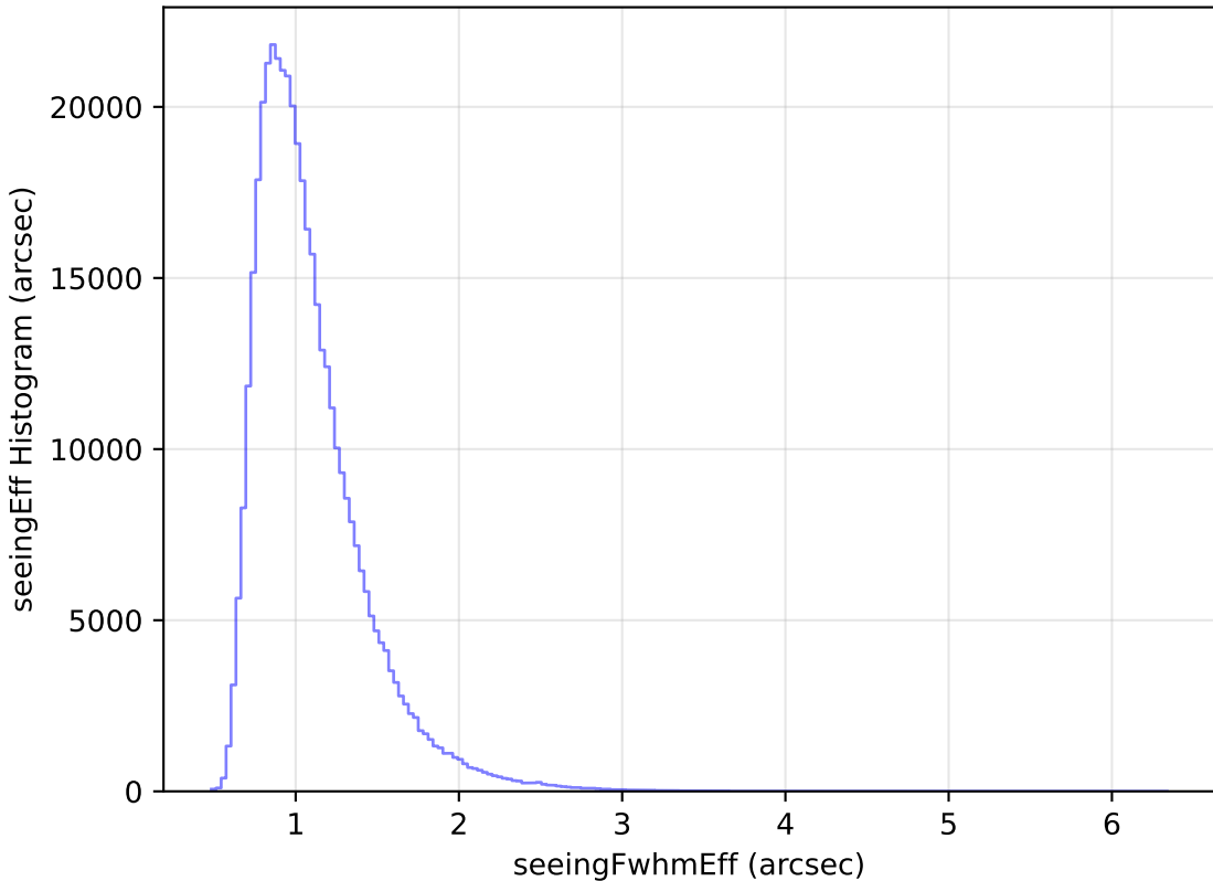
ddf_loaded_half_fl2_v3.4_10yrs WFD z band: seeingEff Histogram
