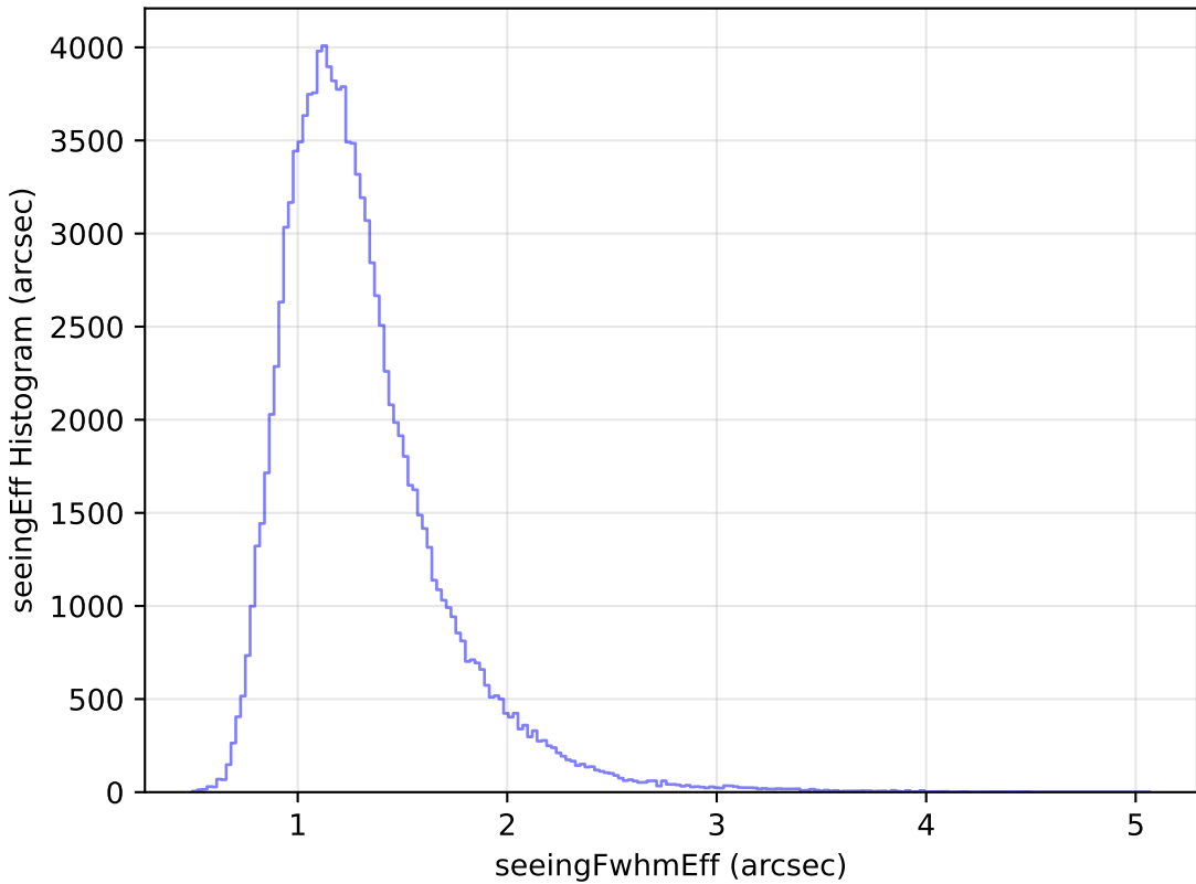
ddf_loaded_half_fl2_v3.4_10yrs WFD u band: seeingEff Histogram
