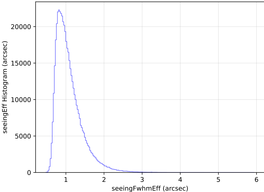
ddf_loaded_half_fl2_v3.4_10yrs WFD i band: seeingEff Histogram
