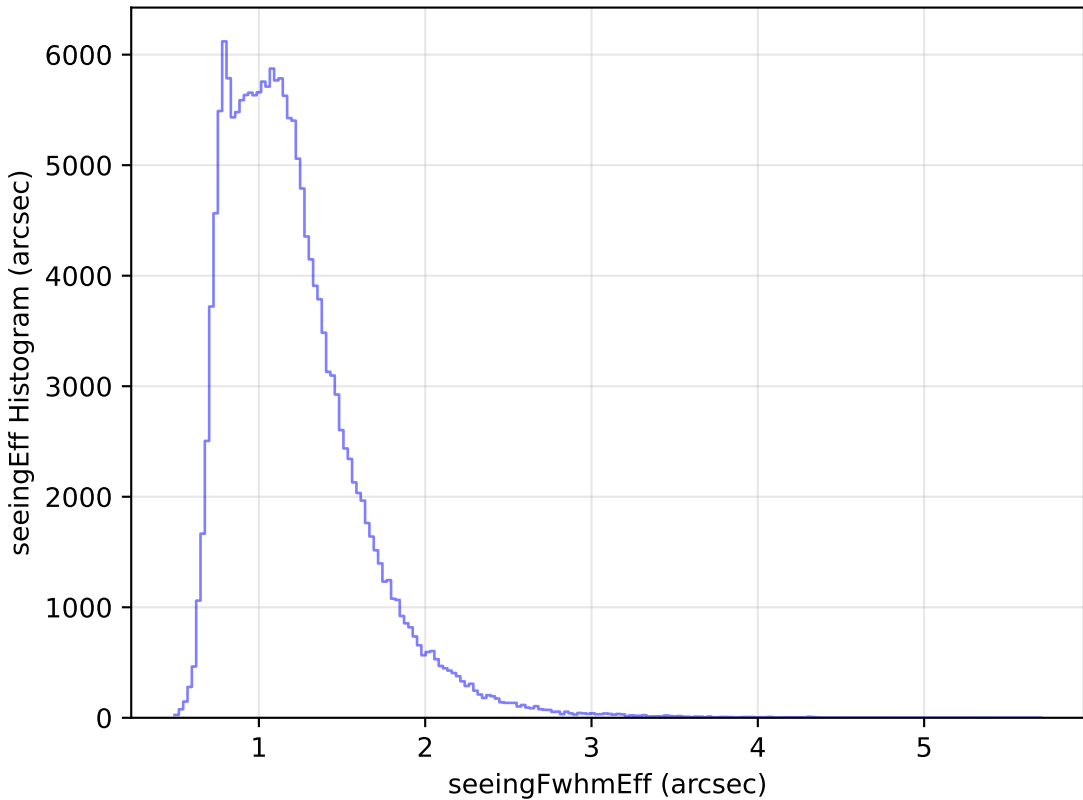
ddf_loaded_half_fl2_v3.4_10yrs WFD g band: seeingEff Histogram
