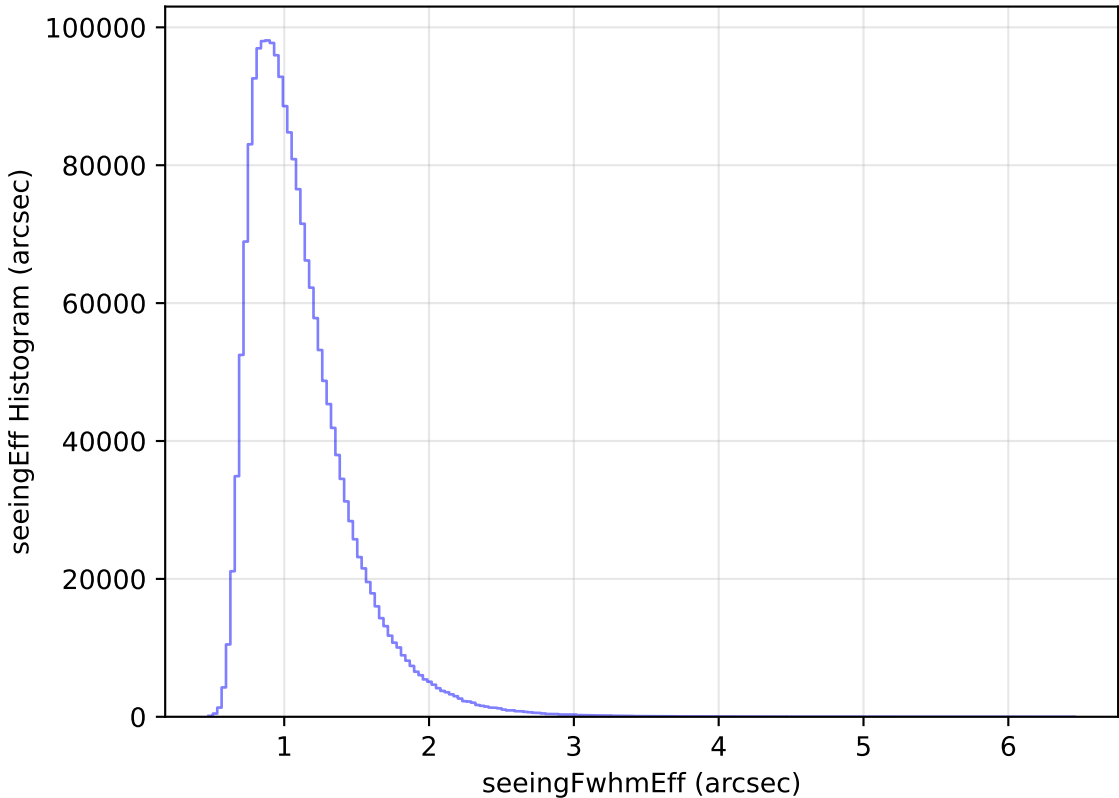
ddf_loaded_half_fl2_v3.4_10yrs WFD all bands: seeingEff Histogram
