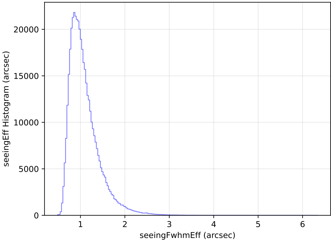
ddf_loaded_half_fl2_v3.4_10yrs All sky z band: seeingEff Histogram
