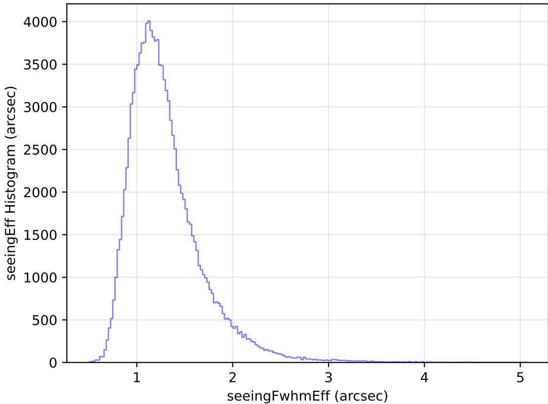
ddf_loaded_half_fl2_v3.4_10yrs All sky u band: seeingEff Histogram
