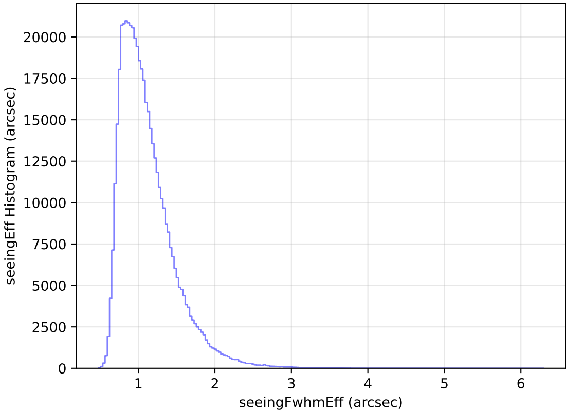
ddf_loaded_half_fl2_v3.4_10yrs All sky r band: seeingEff Histogram
