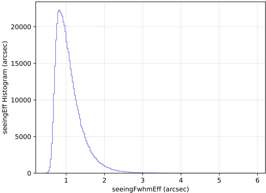
ddf_loaded_half_fl2_v3.4_10yrs All sky i band: seeingEff Histogram
