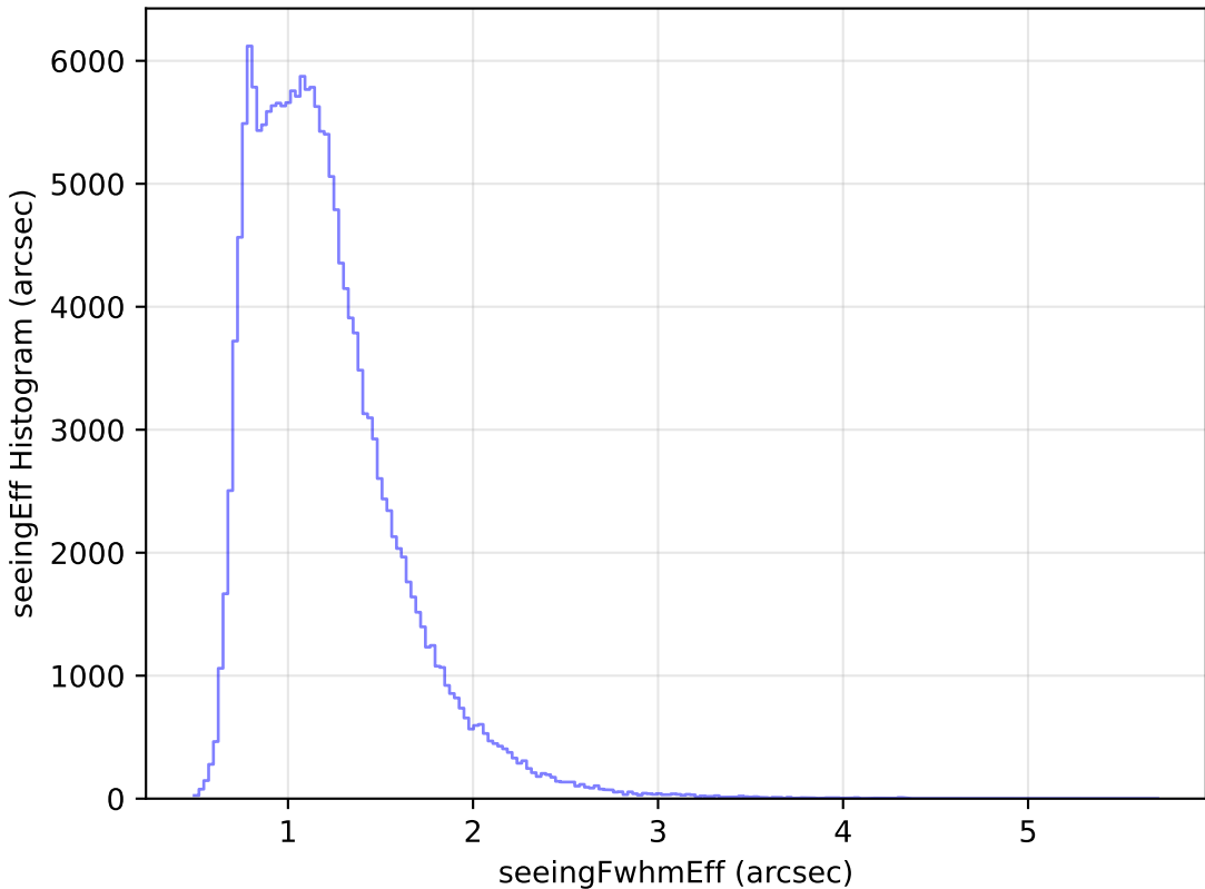
ddf_loaded_half_fl2_v3.4_10yrs All sky g band: seeingEff Histogram
