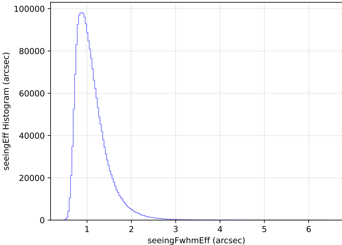
ddf_loaded_half_fl2_v3.4_10yrs All sky all bands: seeingEff Histogram
