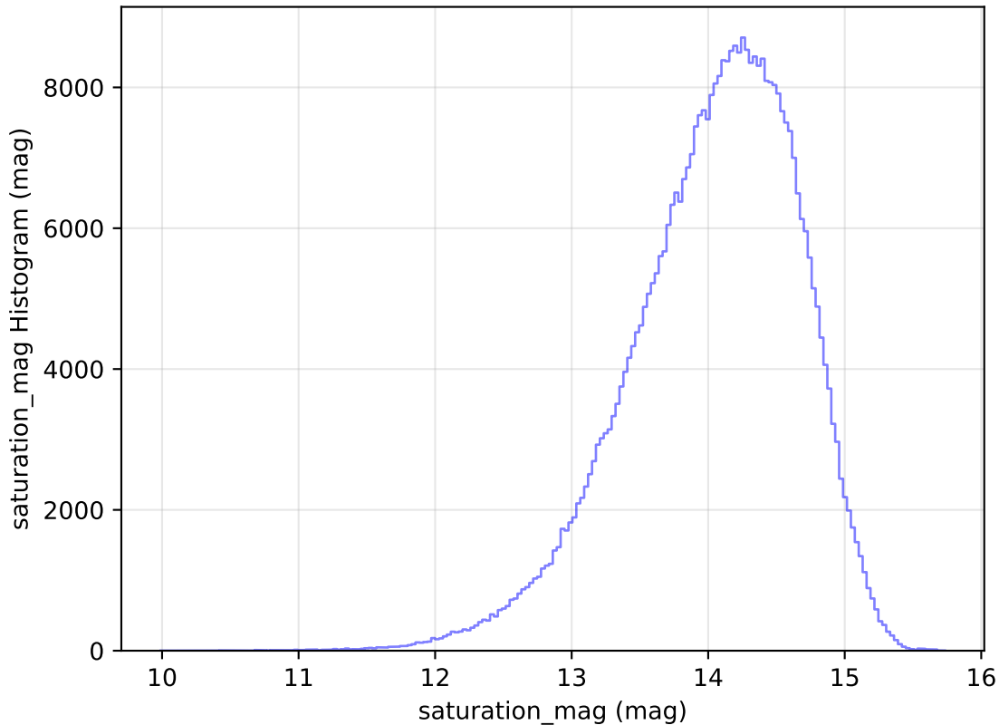
ddf_loaded_half_fl2_v3.4_10yrs WFD z band: saturation_mag Histogram
