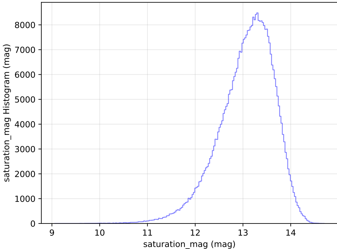
ddf_loaded_half_fl2_v3.4_10yrs WFD y band: saturation_mag Histogram
