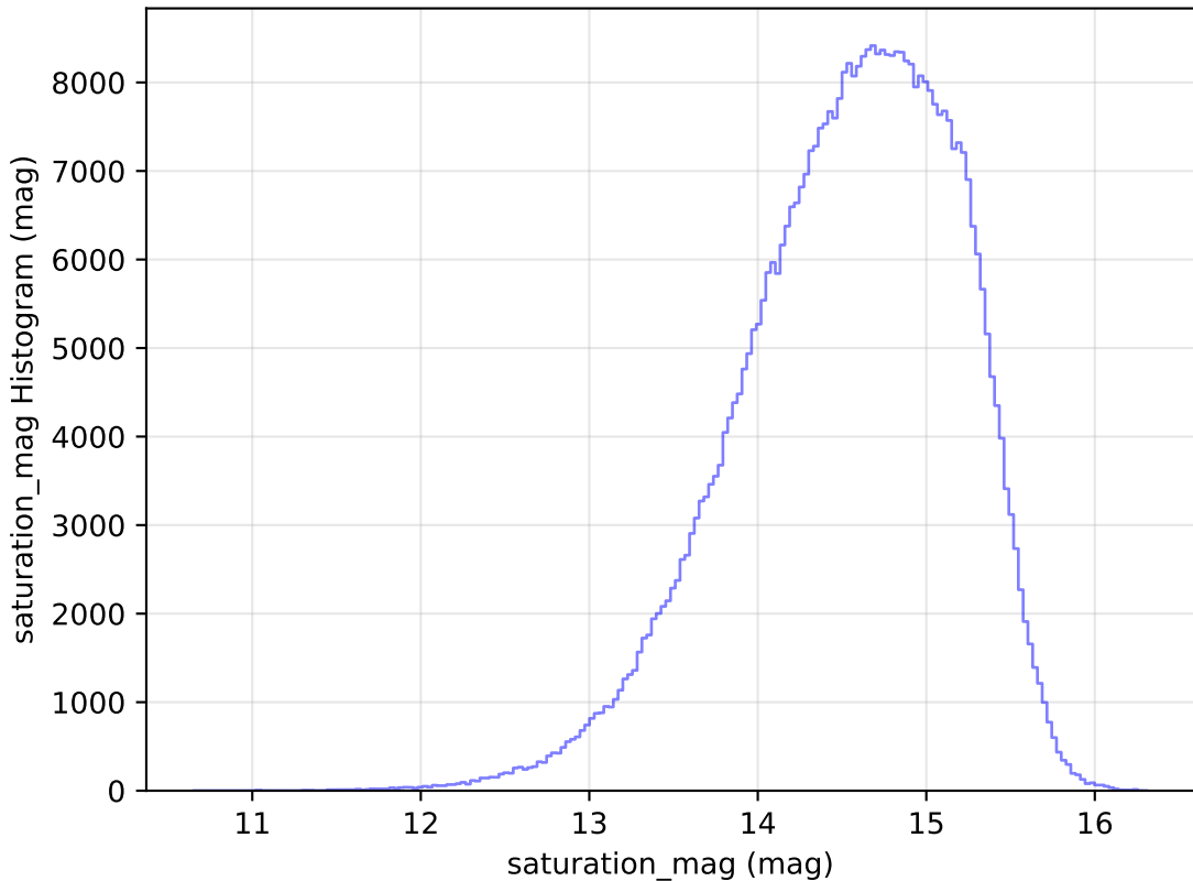
ddf_loaded_half_fl2_v3.4_10yrs WFD r band: saturation_mag Histogram
