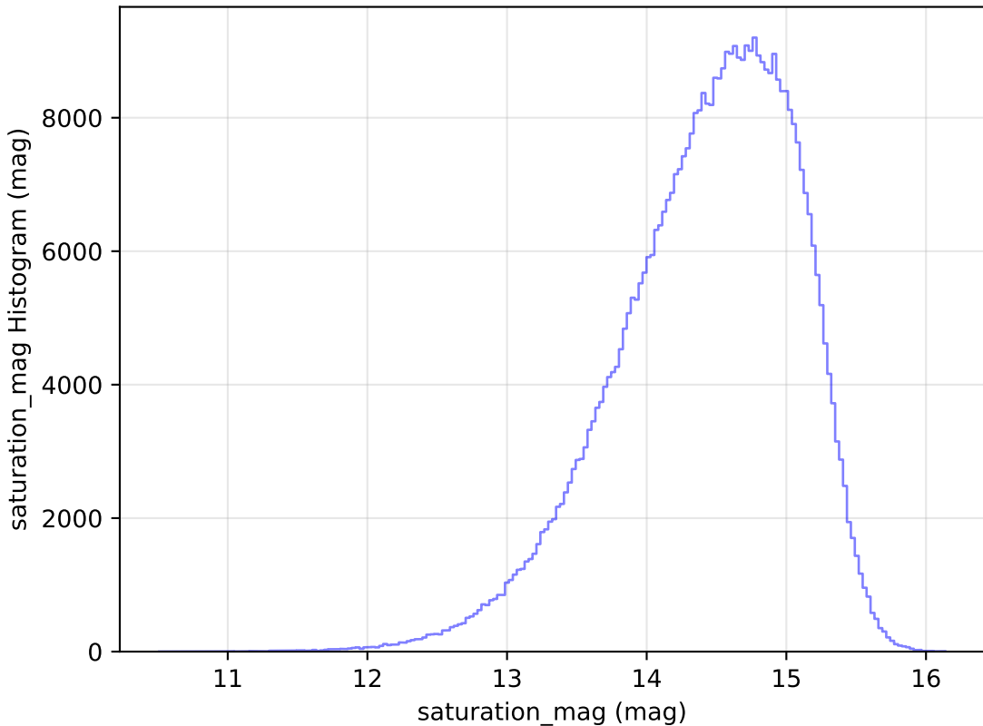
ddf_loaded_half_fl2_v3.4_10yrs WFD i band: saturation_mag Histogram
