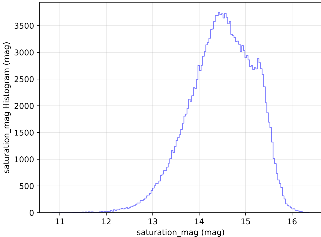
ddf_loaded_half_fl2_v3.4_10yrs WFD g band: saturation_mag Histogram
