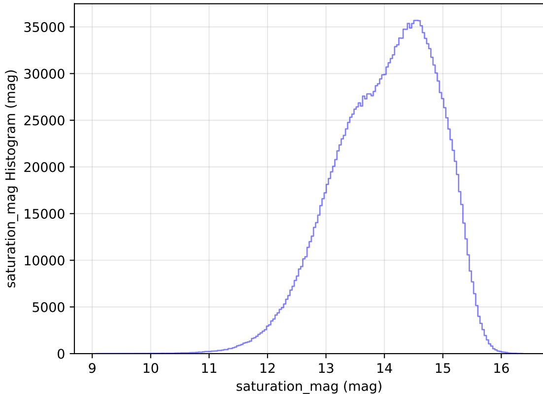
ddf_loaded_half_fl2_v3.4_10yrs WFD all bands: saturation_mag Histogram
