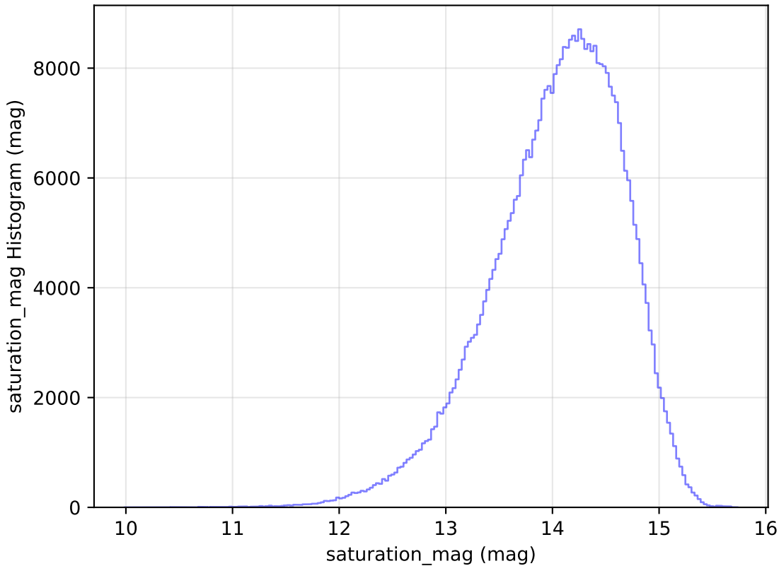
ddf_loaded_half_fl2_v3.4_10yrs All sky z band: saturation_mag Histogram
