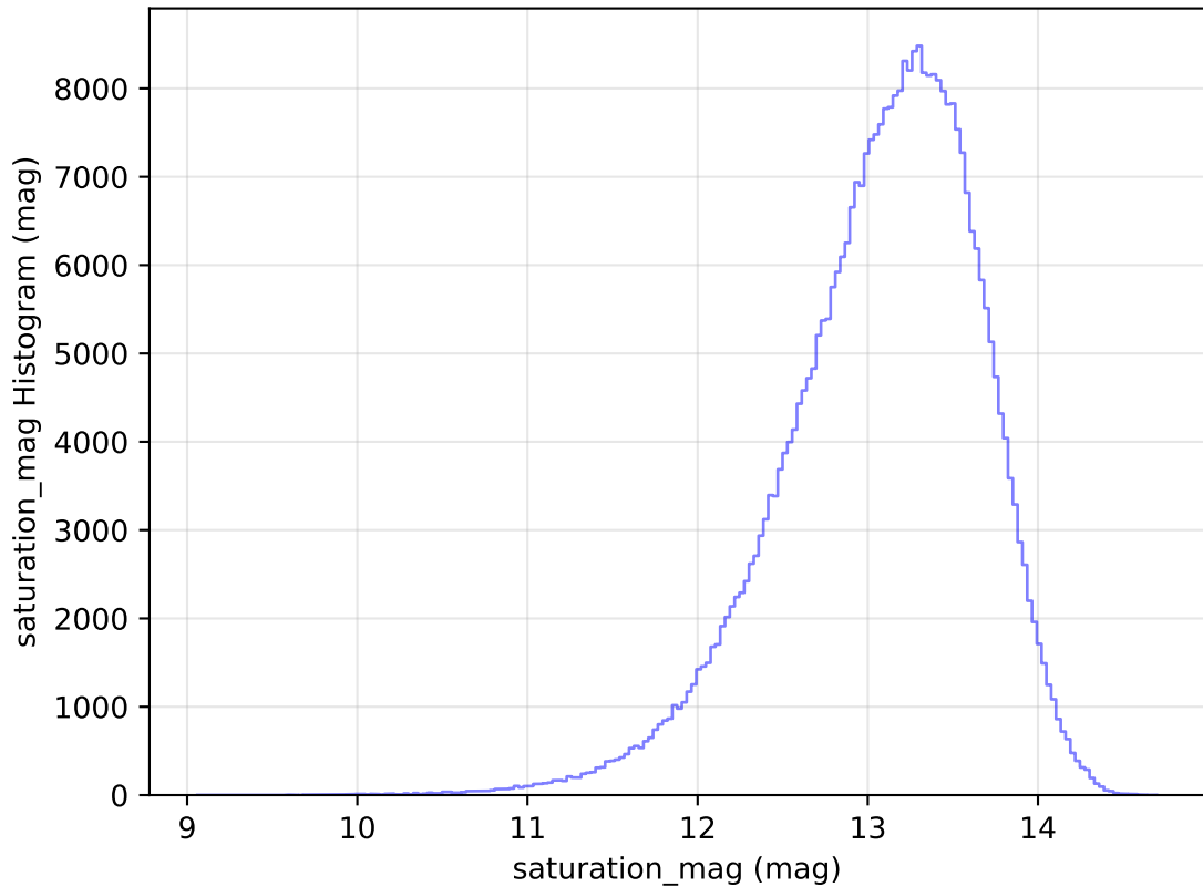
ddf_loaded_half_fl2_v3.4_10yrs All sky y band: saturation_mag Histogram
