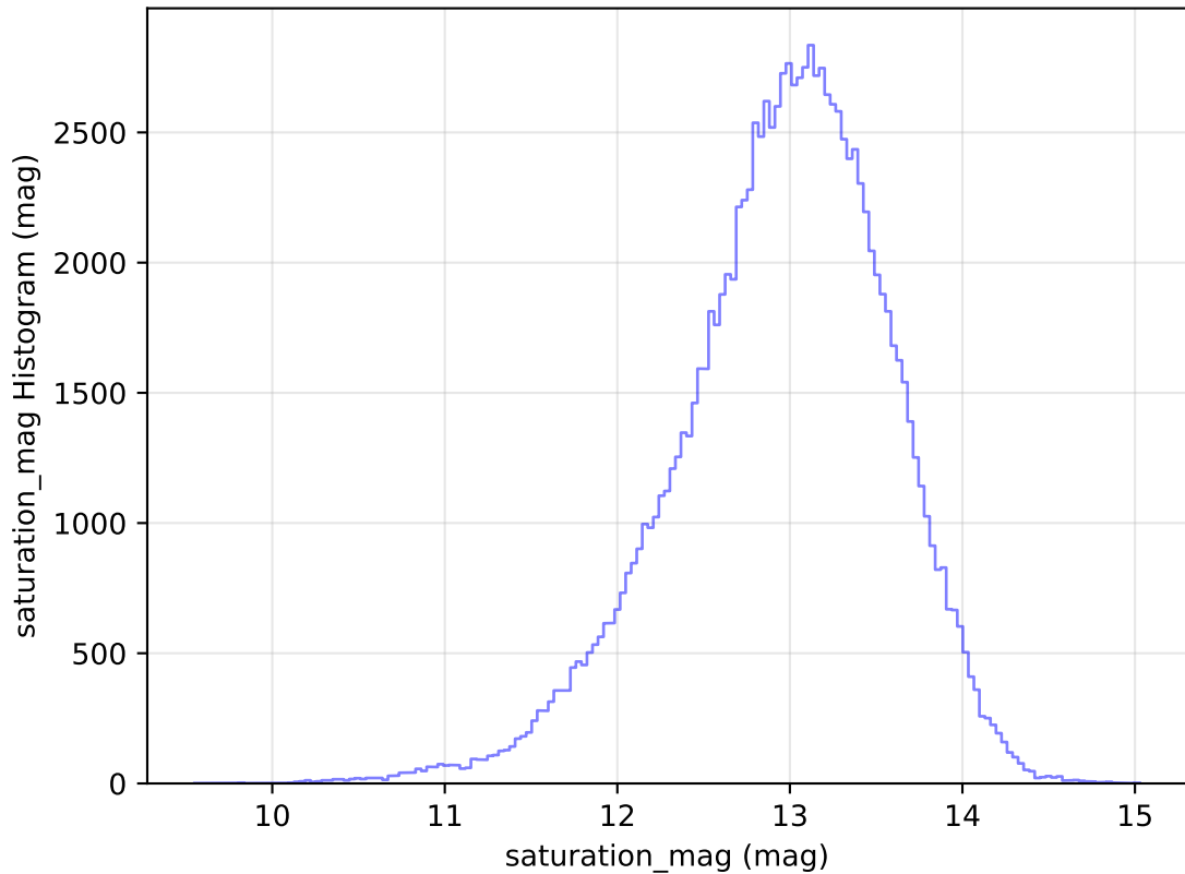
ddf_loaded_half_fl2_v3.4_10yrs All sky u band: saturation_mag Histogram
