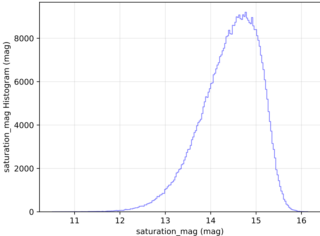
ddf_loaded_half_fl2_v3.4_10yrs All sky i band: saturation_mag Histogram
