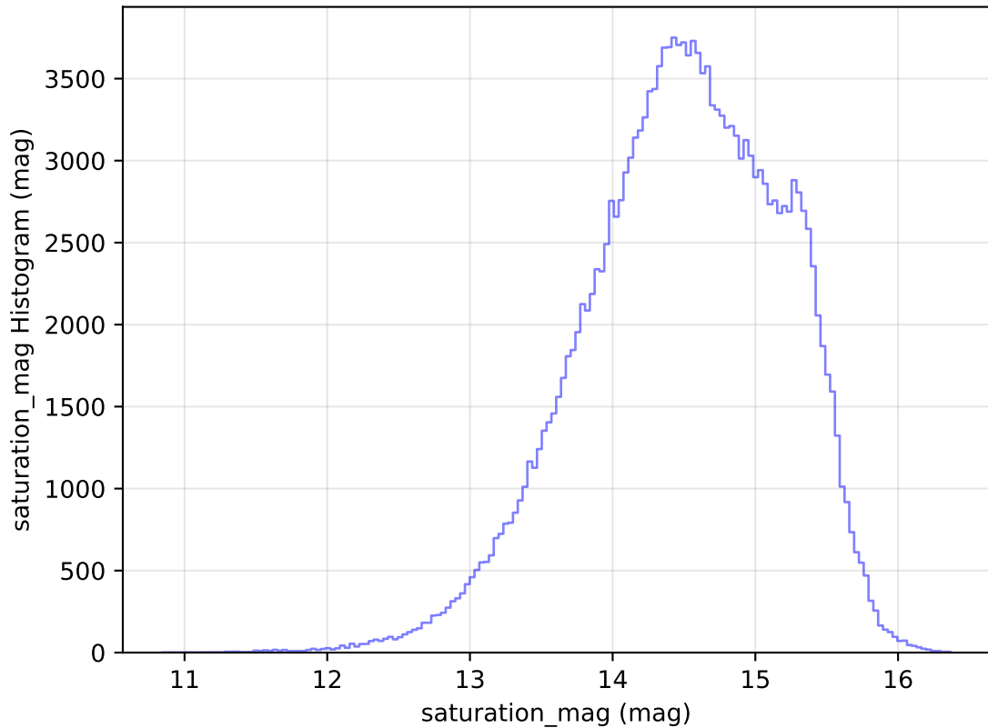
ddf_loaded_half_fl2_v3.4_10yrs All sky g band: saturation_mag Histogram
