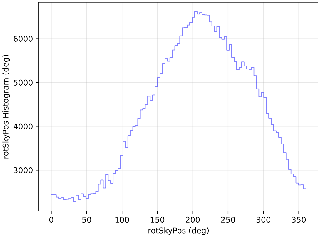
ddf_loaded_half_fl2_v3.4_10yrs WFD z band: rotSkyPos Histogram
