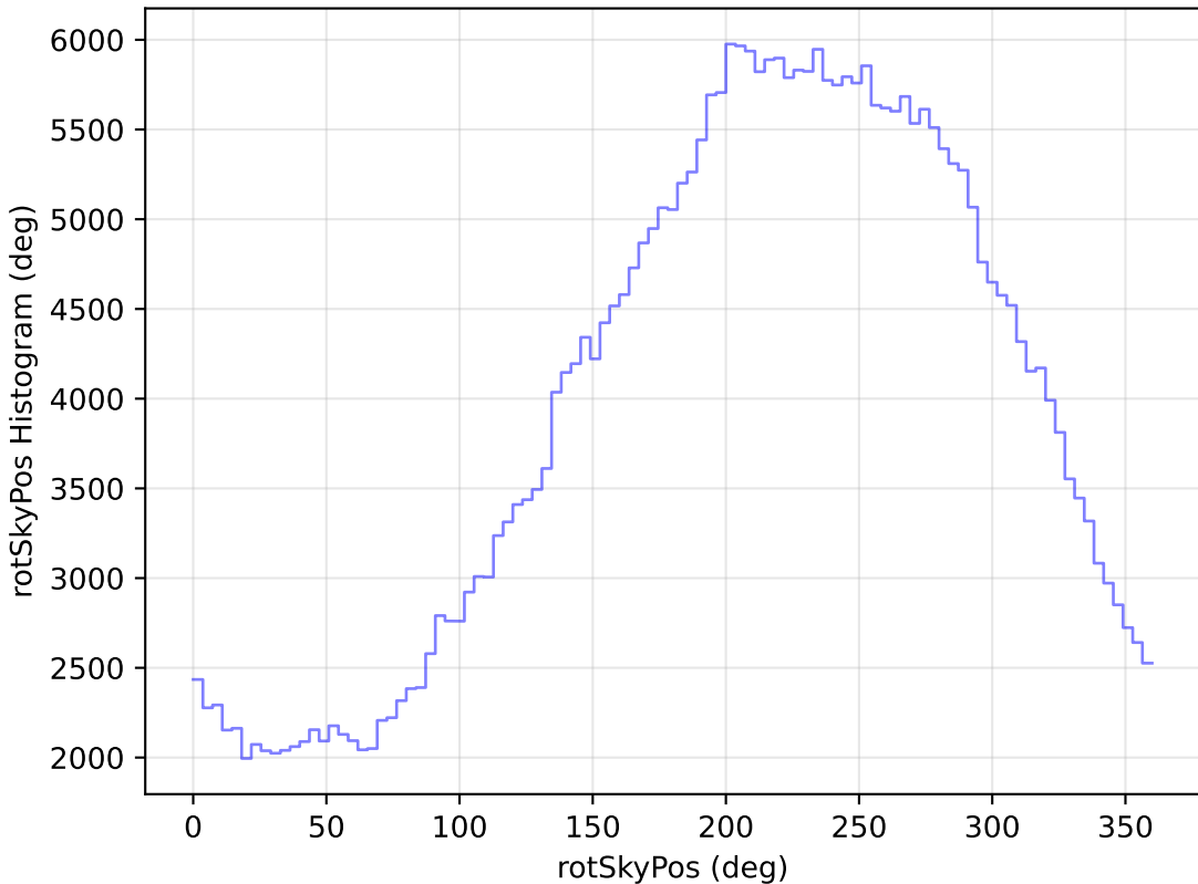
ddf_loaded_half_fl2_v3.4_10yrs WFD y band: rotSkyPos Histogram
