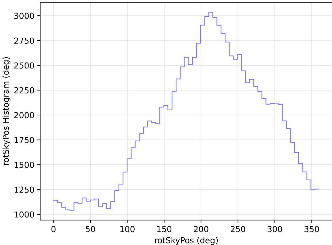
ddf_loaded_half_fl2_v3.4_10yrs WFD u band: rotSkyPos Histogram
