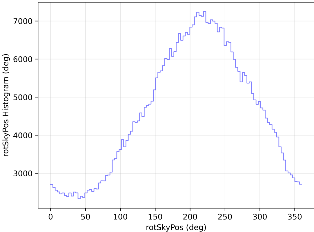
ddf_loaded_half_fl2_v3.4_10yrs WFD i band: rotSkyPos Histogram
