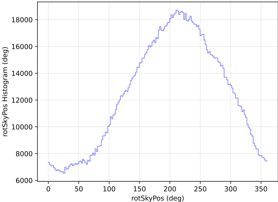
ddf_loaded_half_fl2_v3.4_10yrs WFD all bands: rotSkyPos Histogram
