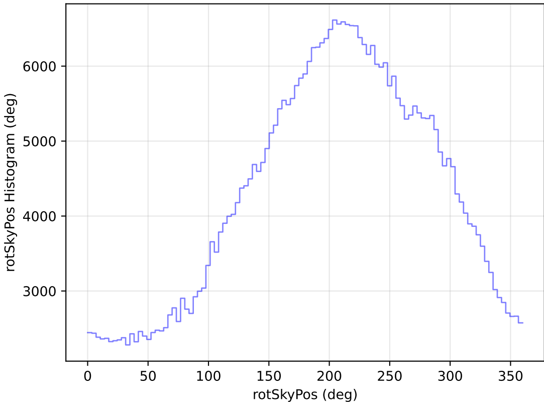
ddf_loaded_half_fl2_v3.4_10yrs All sky z band: rotSkyPos Histogram
