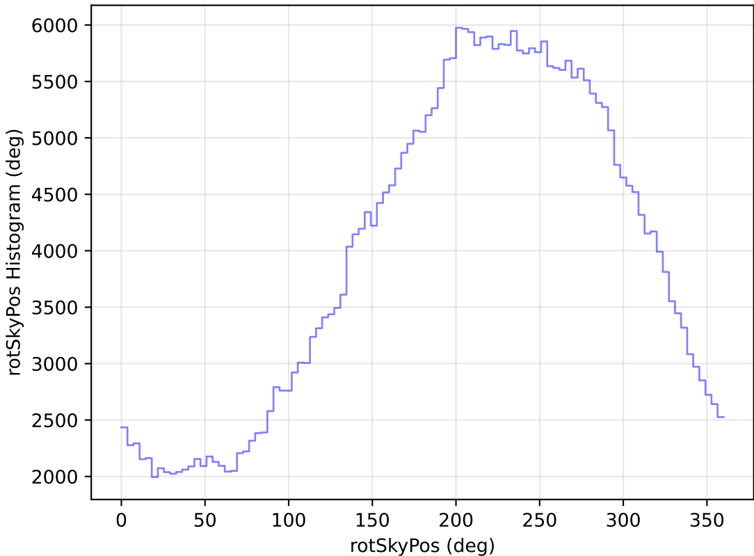
ddf_loaded_half_fl2_v3.4_10yrs All sky y band: rotSkyPos Histogram
