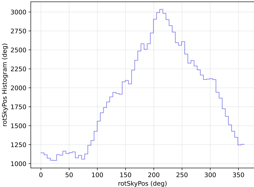
ddf_loaded_half_fl2_v3.4_10yrs All sky u band: rotSkyPos Histogram
