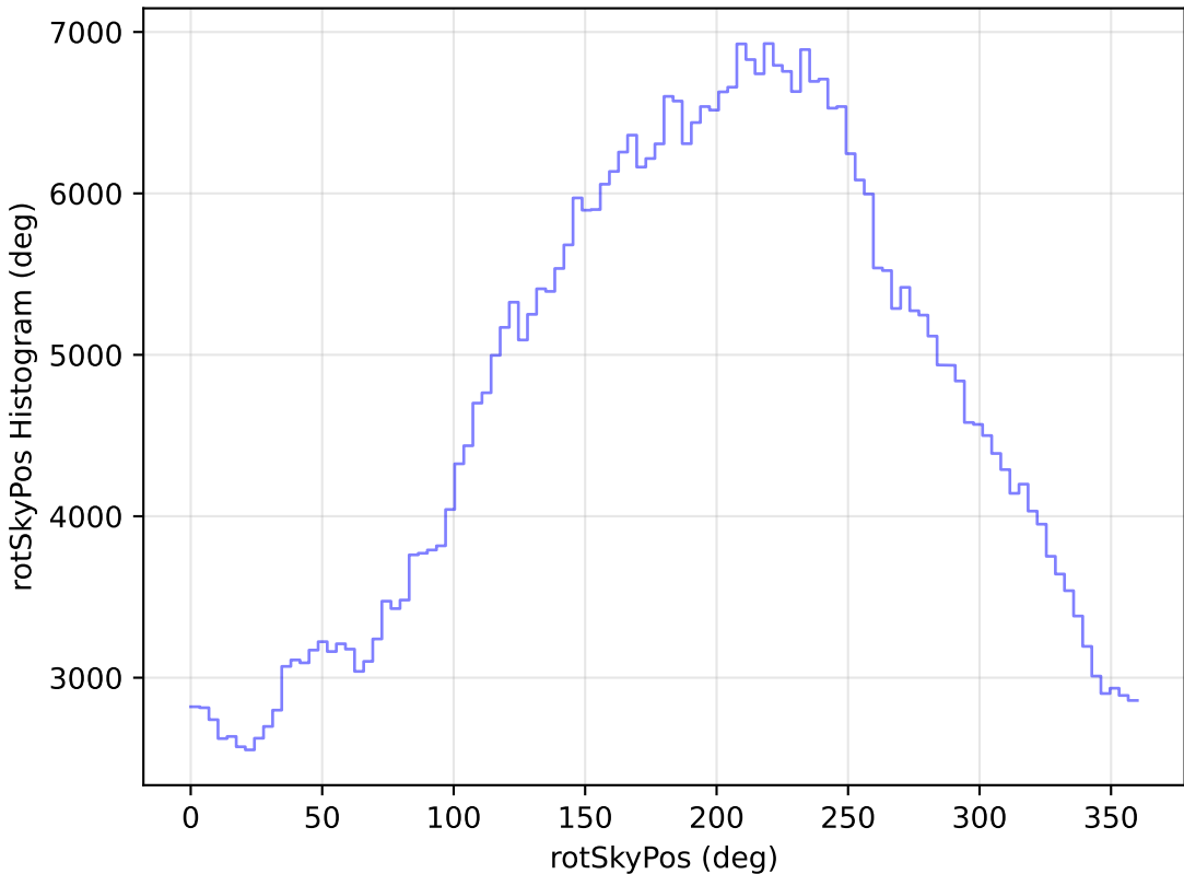
ddf_loaded_half_fl2_v3.4_10yrs All sky r band: rotSkyPos Histogram
