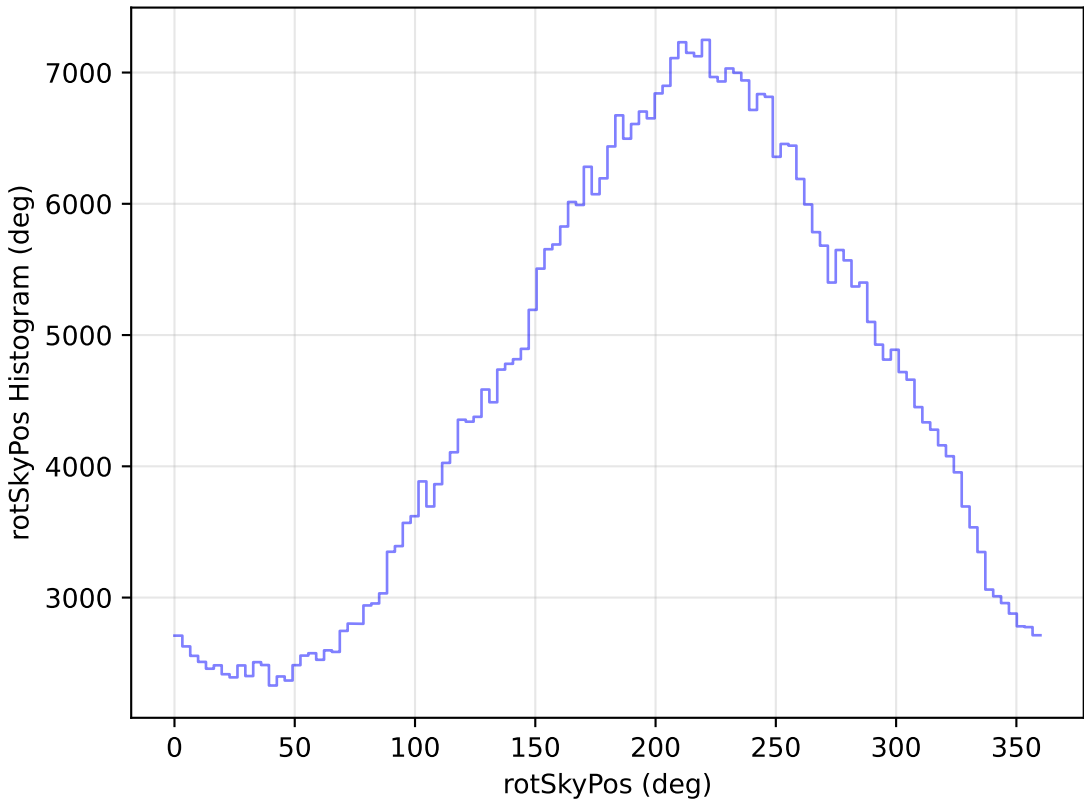
ddf_loaded_half_fl2_v3.4_10yrs All sky i band: rotSkyPos Histogram
