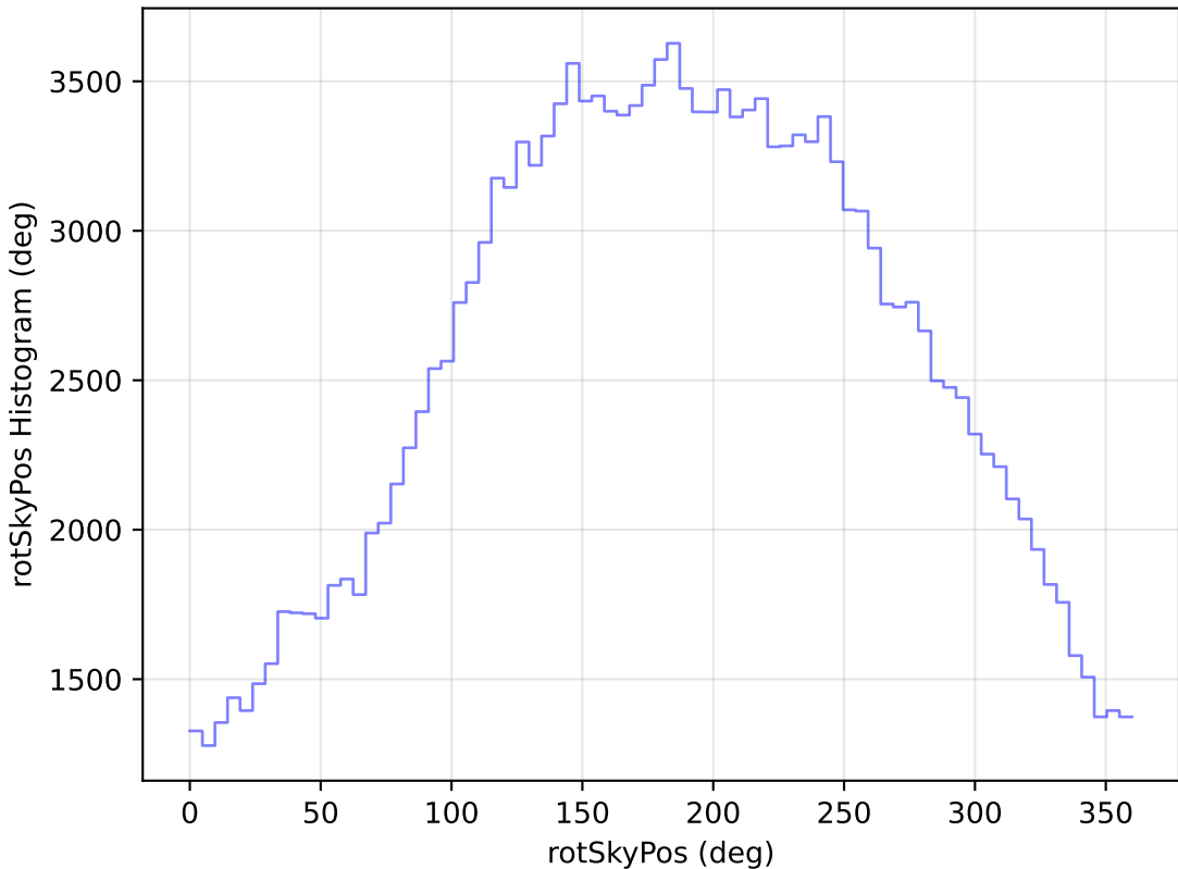
ddf_loaded_half_fl2_v3.4_10yrs All sky g band: rotSkyPos Histogram
