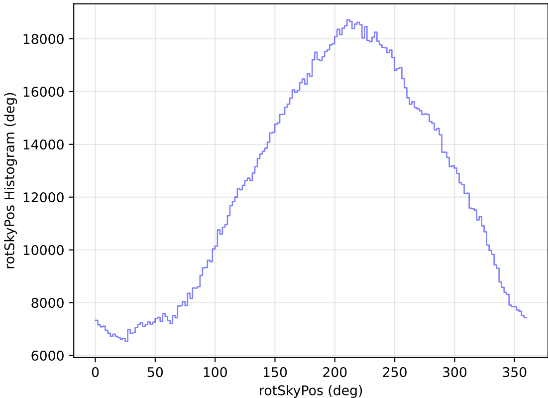
ddf_loaded_half_fl2_v3.4_10yrs All sky all bands: rotSkyPos Histogram
