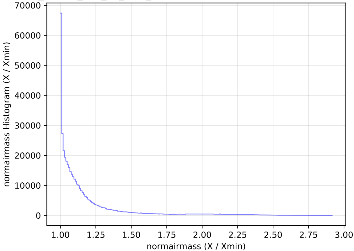
ddf_loaded_half_fl2_v3.4_10yrs WFD z band: normairmass Histogram
