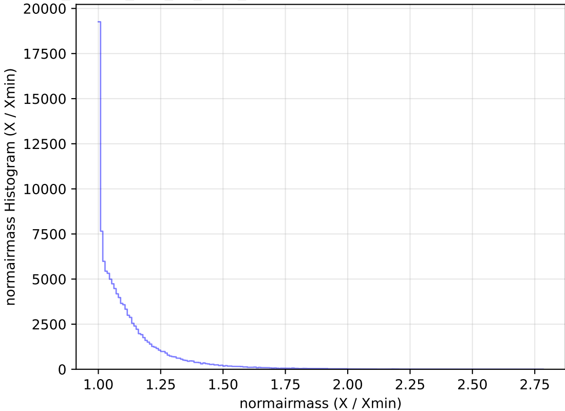
ddf_loaded_half_fl2_v3.4_10yrs WFD u band: normairmass Histogram
