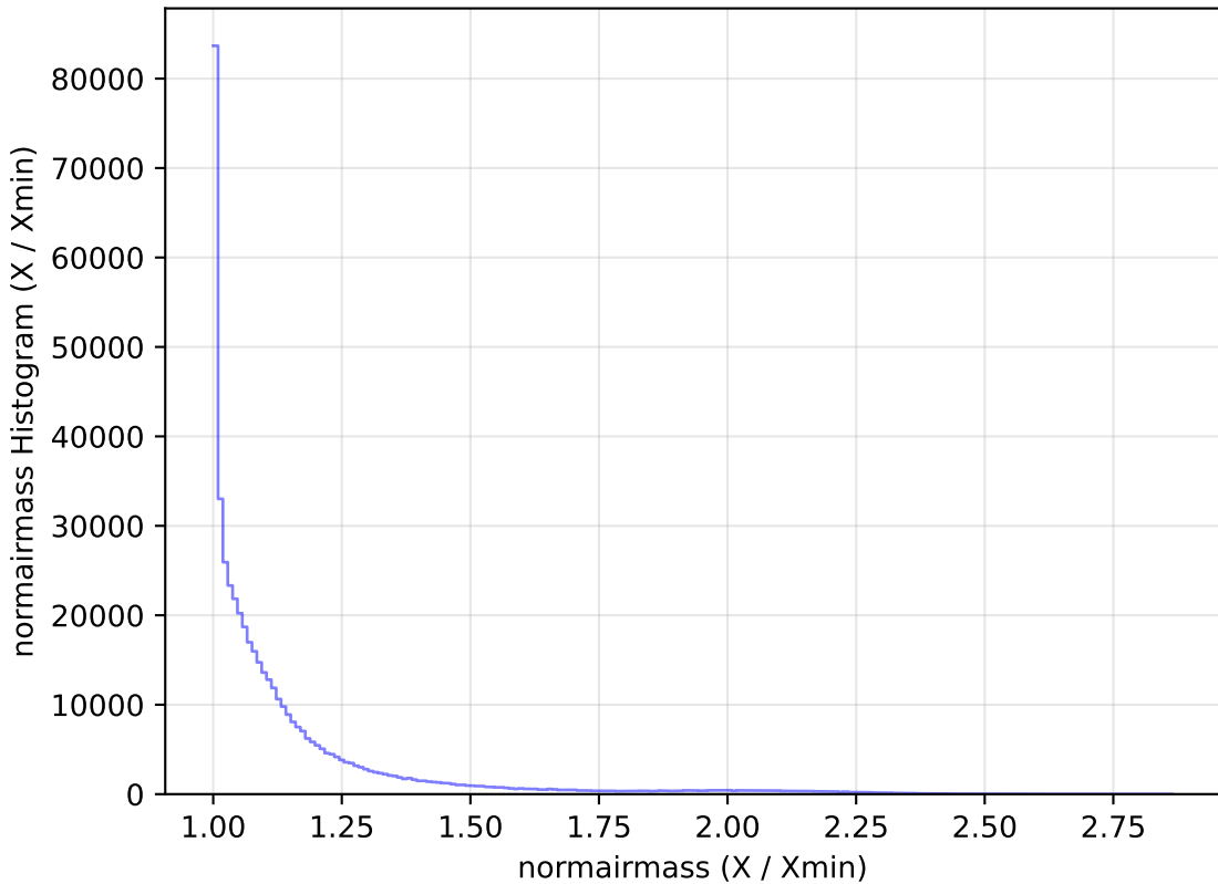
ddf_loaded_half_fl2_v3.4_10yrs WFD r band: normairmass Histogram
