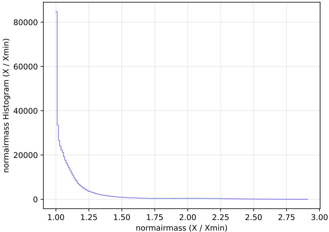
ddf_loaded_half_fl2_v3.4_10yrs WFD i band: normairmass Histogram
