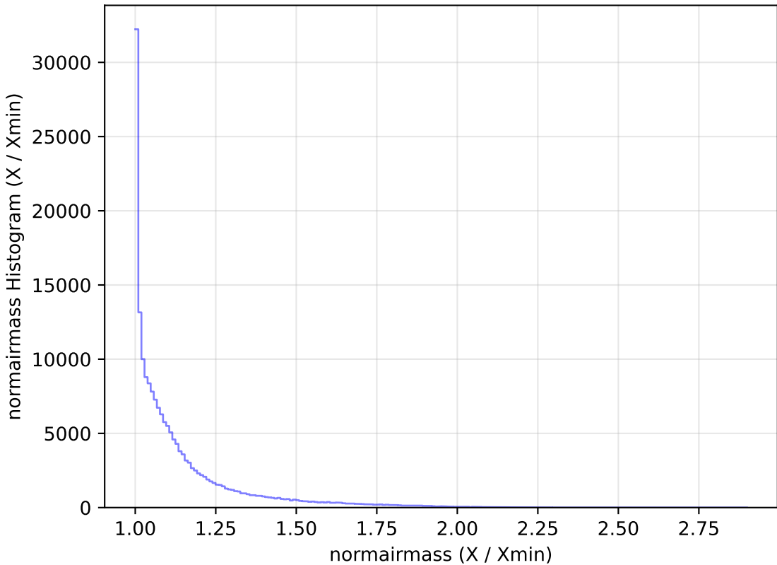
ddf_loaded_half_fl2_v3.4_10yrs WFD g band: normairmass Histogram
