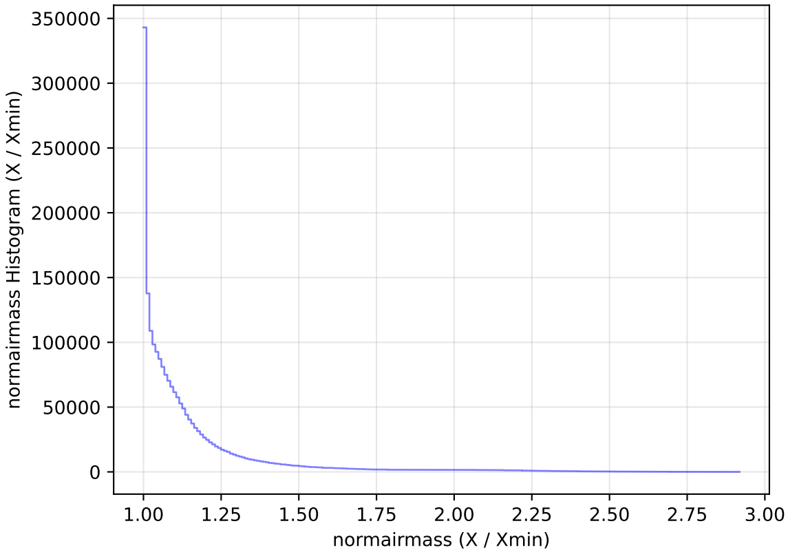
ddf_loaded_half_fl2_v3.4_10yrs WFD all bands: normairmass Histogram
