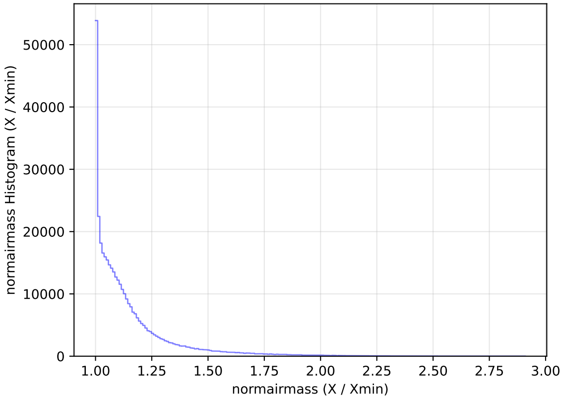
ddf_loaded_half_fl2_v3.4_10yrs All sky y band: normairmass Histogram
