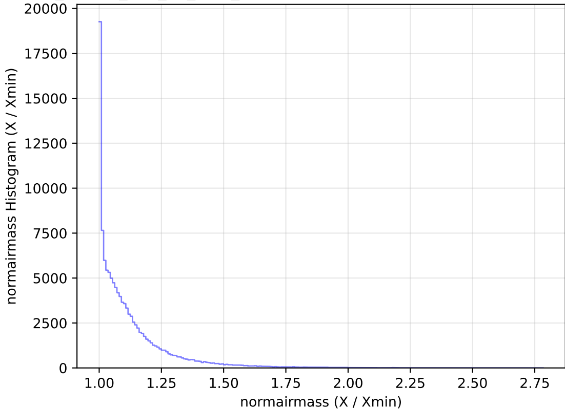
ddf_loaded_half_fl2_v3.4_10yrs All sky u band: normairmass Histogram
