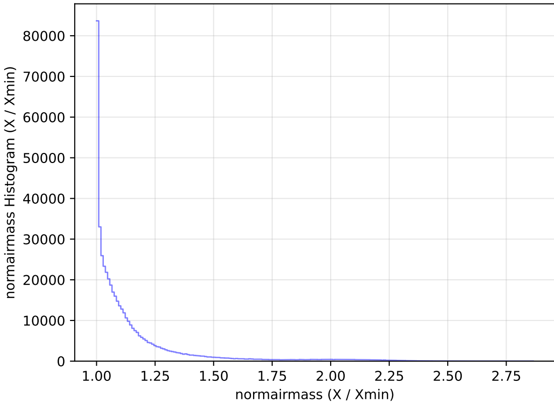
ddf_loaded_half_fl2_v3.4_10yrs All sky r band: normairmass Histogram
